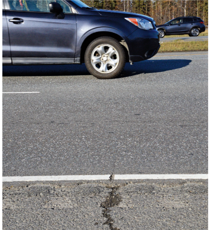
In late 2019, on busy Glenn Highway, transverse crack in shoulder stops dead at HiMA mix placed two years earlier
